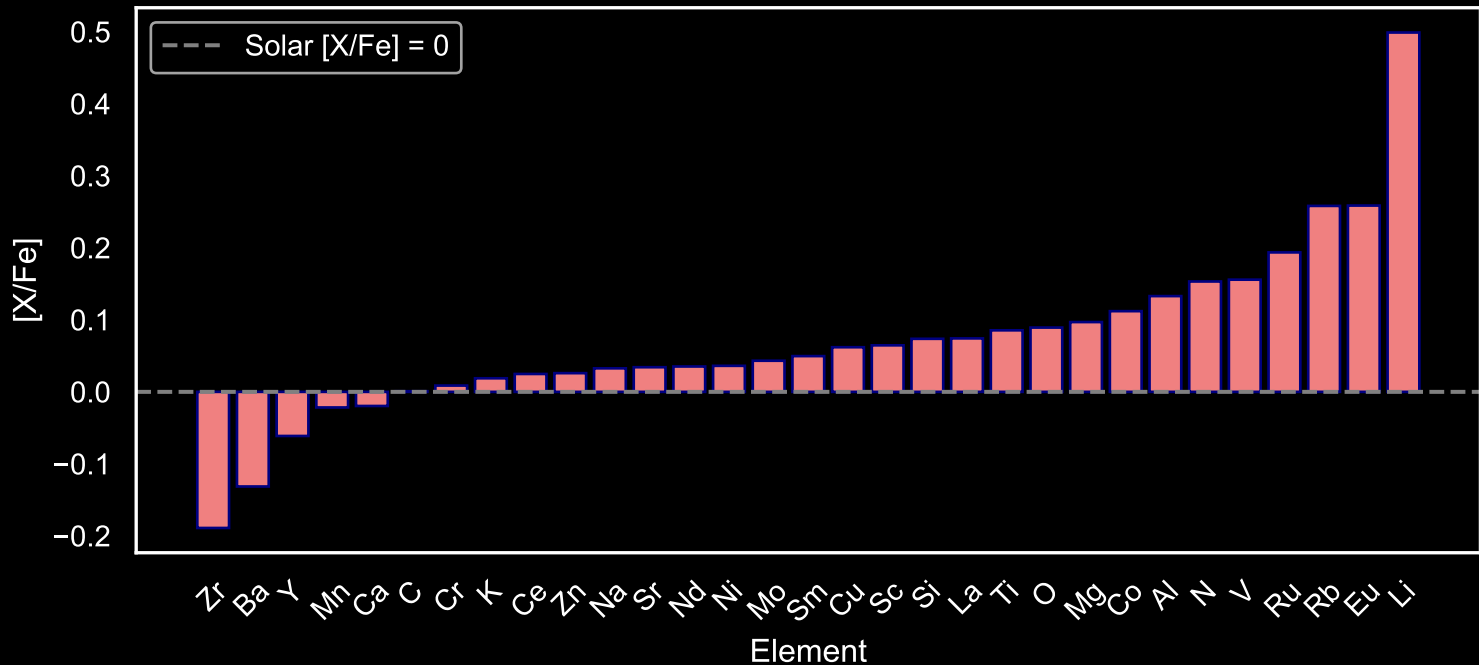
Abundance Pattern for GALAH Star Field [8] (N=205)
