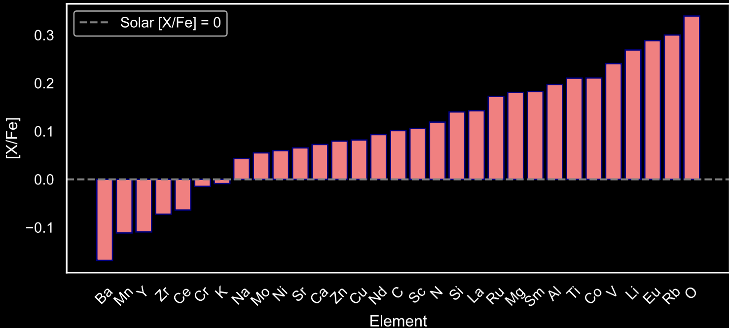
Abundance Pattern for GALAH Red Giants: Star Field [8] (N=44)
