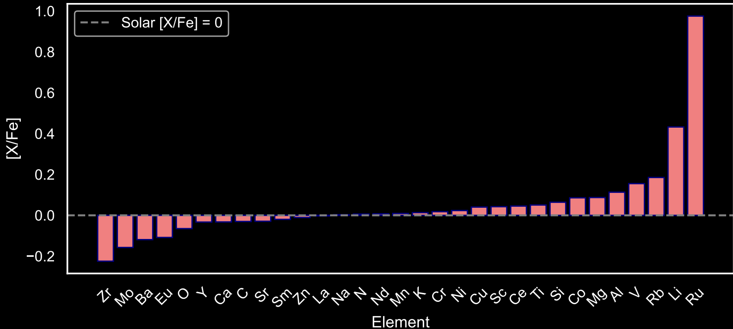
Abundance Pattern for GALAH Main Sequence Stars: Star Field [8] (N=94)
