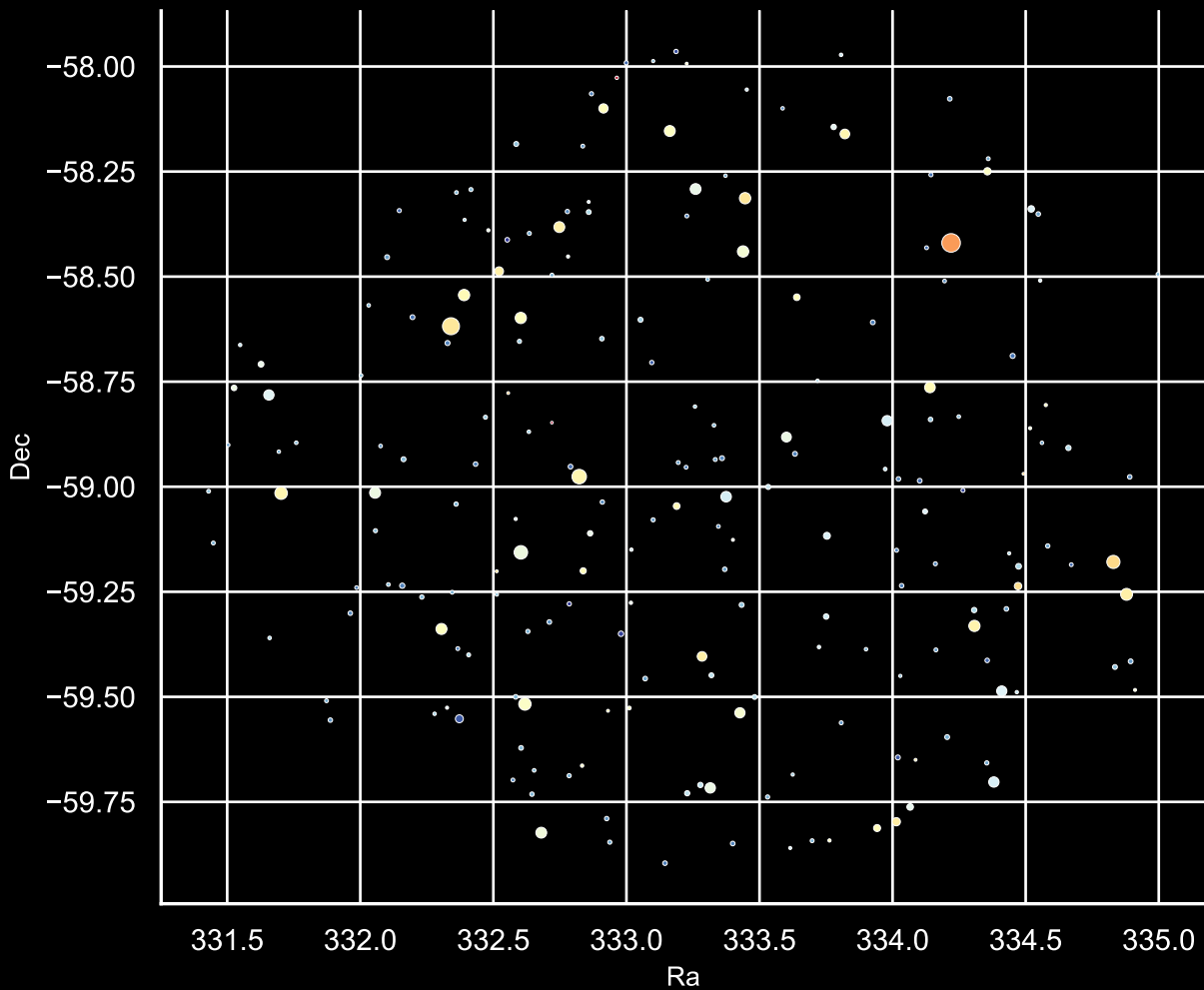
Field [8] Ra [333.23] Dec [-58.99] Stars: 205
