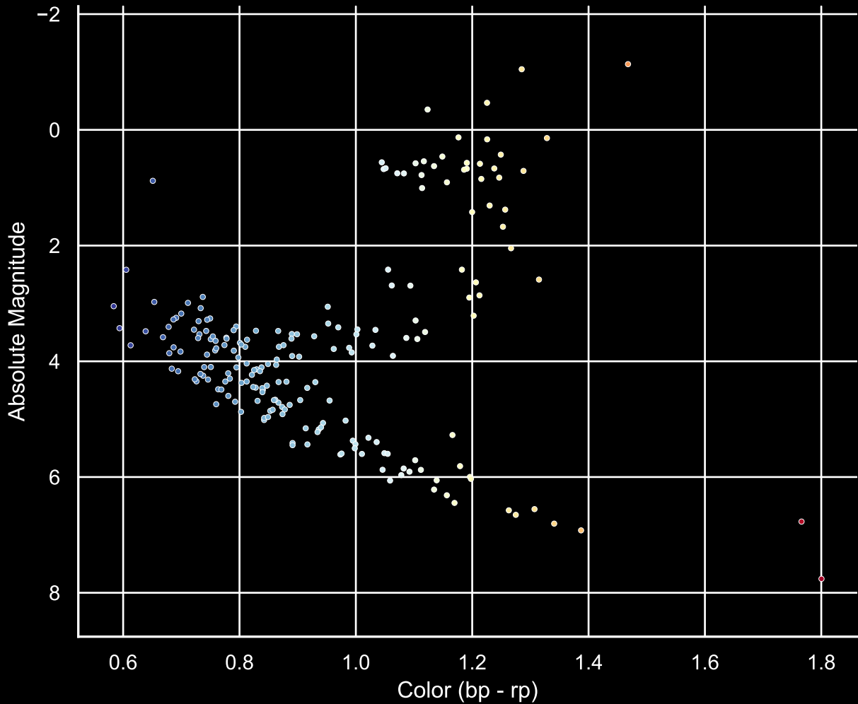
GALAH Hertzprung-Russel Diagram Field [8] Ra [333.23] Dec [-58.99]
