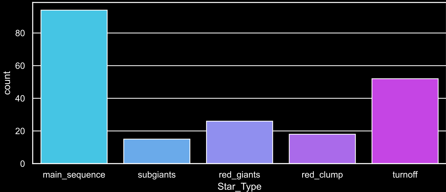
Field [8] Count plot of Star Type
